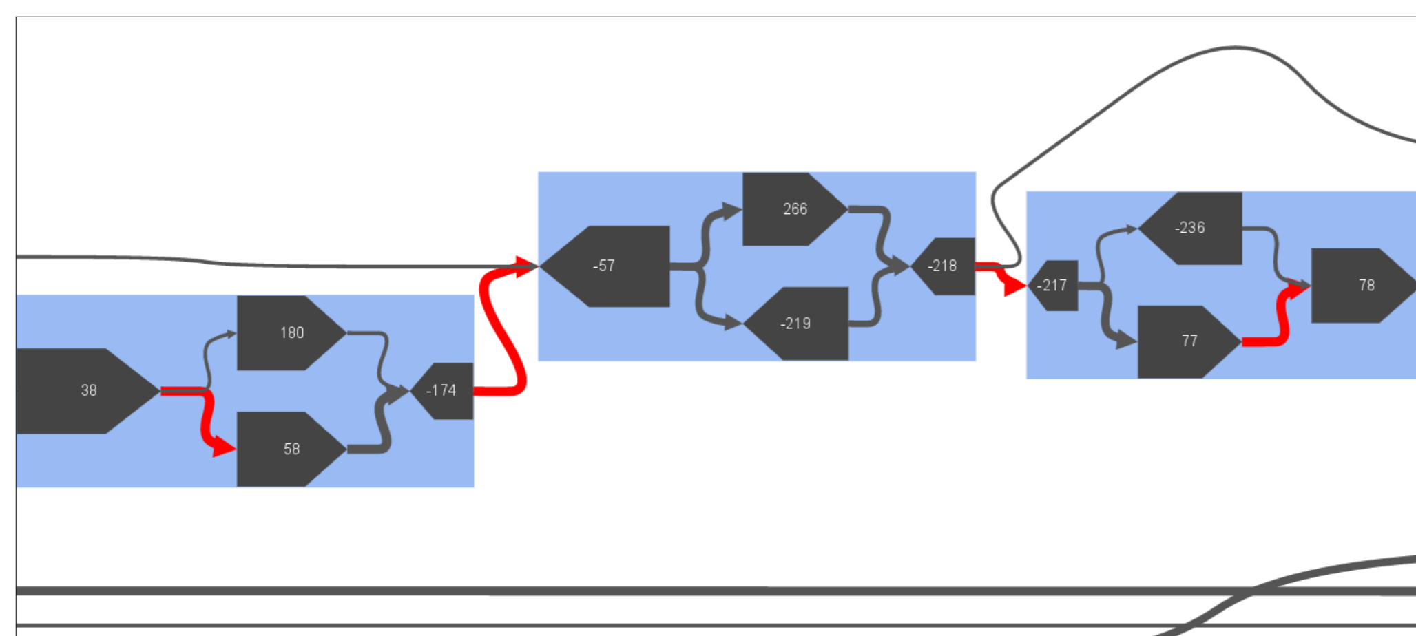
(b) Screenshot captured in MetagenomeScope’s “standard mode” of the same region of the same graph as in Fig. 2a. The collections of contigs highlighted in blue have been flagged as “bubbles,” regions of the assembly graph exhibiting a converge→diverge→converge pattern [4].
