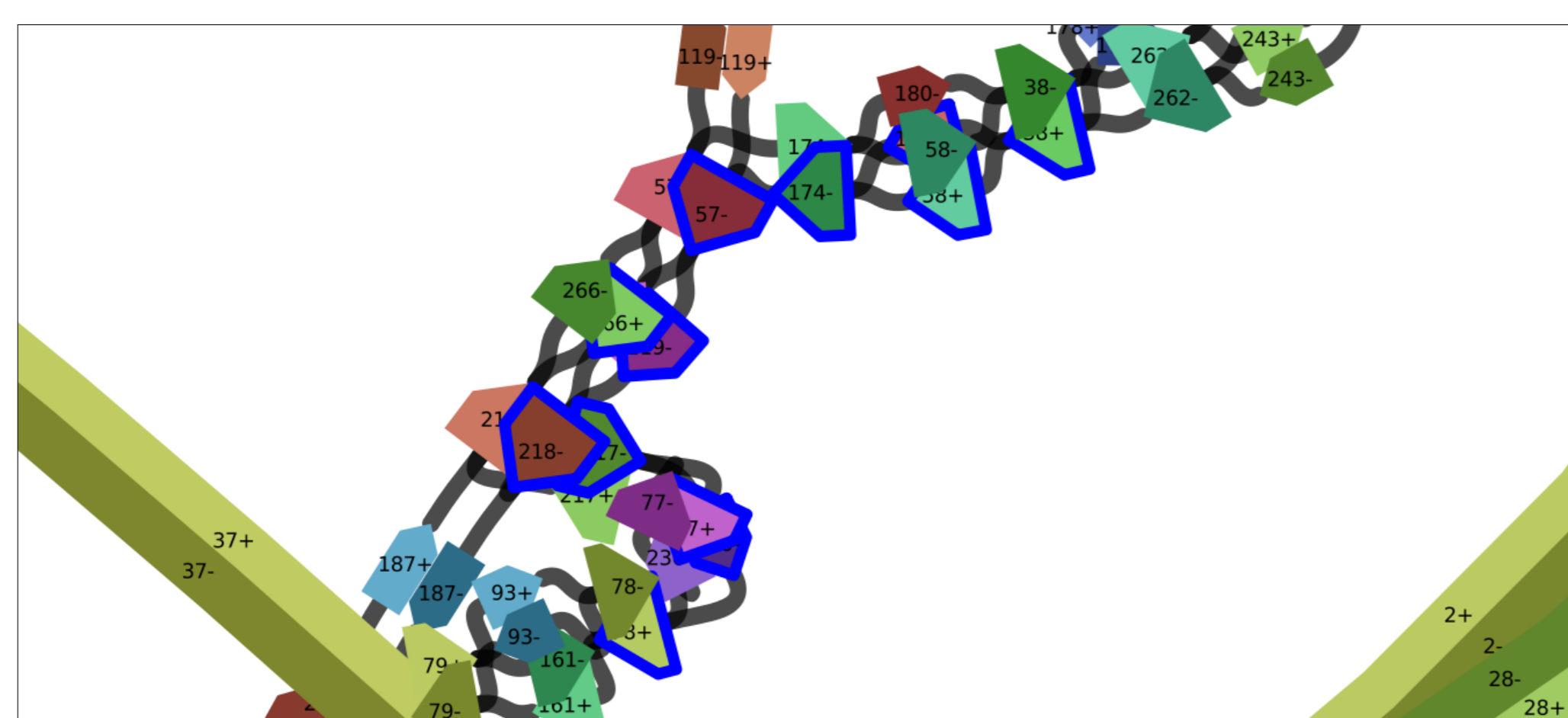
(a) Screenshot captured in Bandage v0.8.1 of a specified region of an E. coli assembly graph. The graph was drawn as a “double graph” in Bandage’s linear layout mode with otherwise default settings. Selected nodes are outlined in blue by Bandage.
